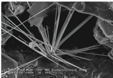
Gypsum: COREX in-house Scanning Electron Microscopy (SEM) photographs above show a variety of scale types
