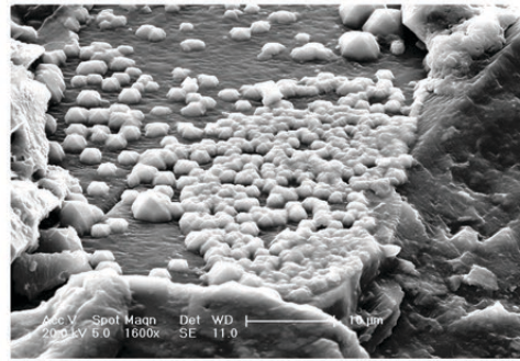
Silica: COREX in-house Scanning Electron Microscopy (SEM) photographs above show a variety of scale types
